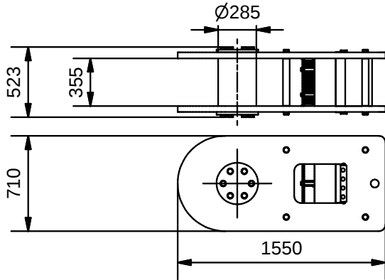
Anchor (1:40)
